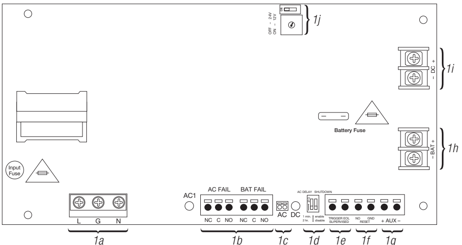
Fig. 1 - eFlowRLBV Configuration
